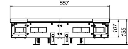
KVU 250-105-135
