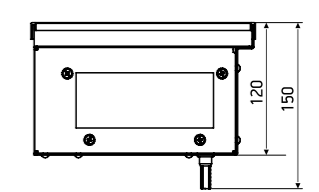
KVU 200-120-90
