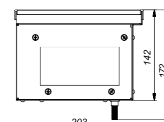
KVU 200-140-90
